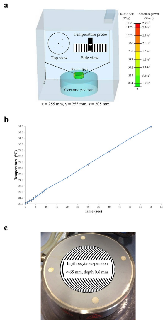
Figure 5. The energy distribution and the exposure system of the 18 GHz EMF. (a) Electric field and absorbed power modeling using CST Microwave Studio 3D Electromagnetic Simulation Software and inset images of the tip positions of the temperature probe in media (top and side view). (b) The heating rate of the RBCs suspension during EMF exposure.
