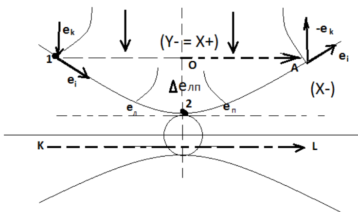
Fig. 6. Quantum of space-matter
