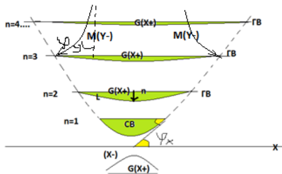
Fig. 7. Quantum gravitational fields.
