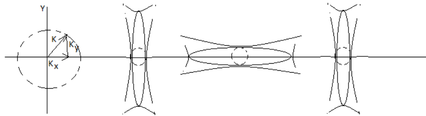
Fig.3. quantum relativistic dynamics of matter space
