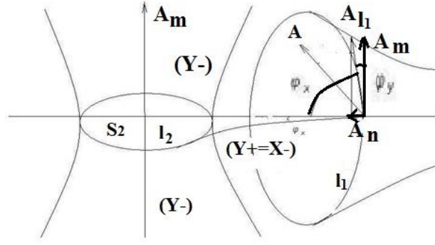
Fig.2. Electro (Y+ = X-) magnetic and gravity (X+ = Y-) mass fields.
