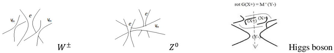
Fig. 8.1.. Electroweak interaction and Higgs boson.
