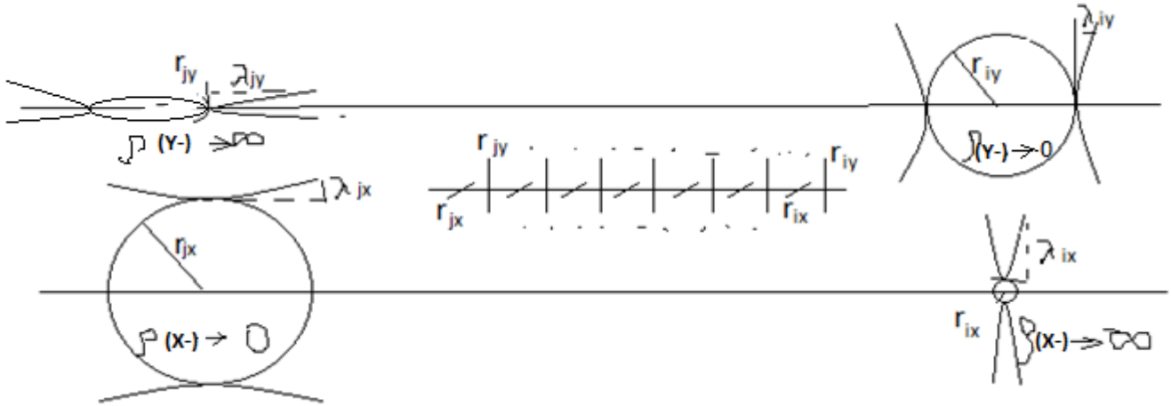
Figure 7.1. The physical vacuum of the Universe
