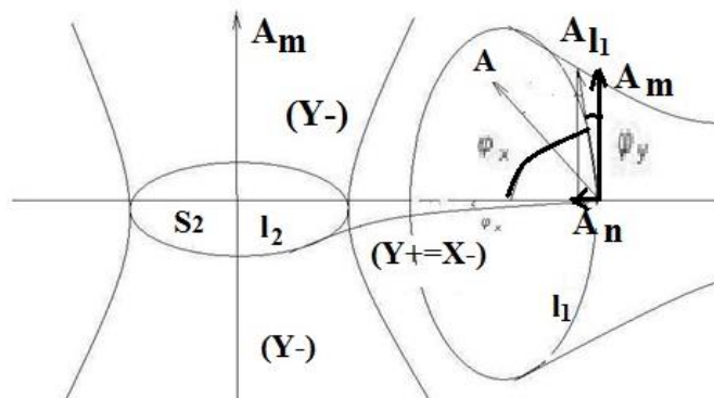
Figure 3. Electro ( Y+ = X- )magnetic and gravitational ( X+ = Y- )fields.
