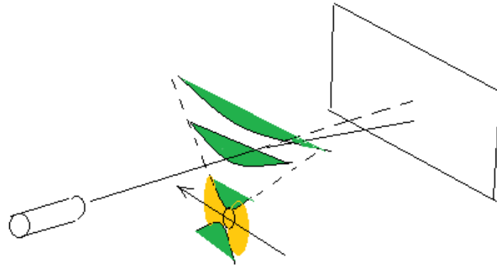
Fig. 5. 4.. Quantum gravity fields.
