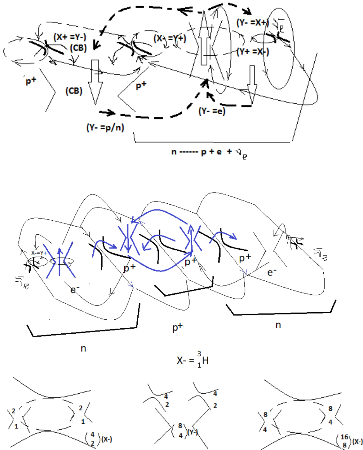
Fig. 9.1. Quantum (Y- = p/n) and similar (Y- = 2n) Strong Interaction Based on these properties (X- = p+) and (X- = \nu_e^-) , the decay time of a neutron in a strong (X-) magnetic field should increase. This is verified in an experiment.
