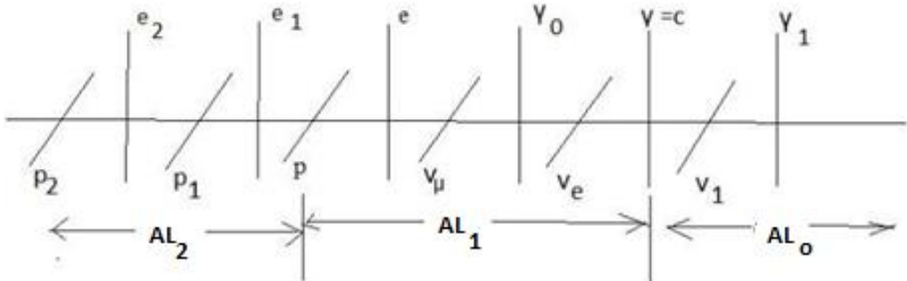
Figure 2. Indivisible quanta of space-matter.
