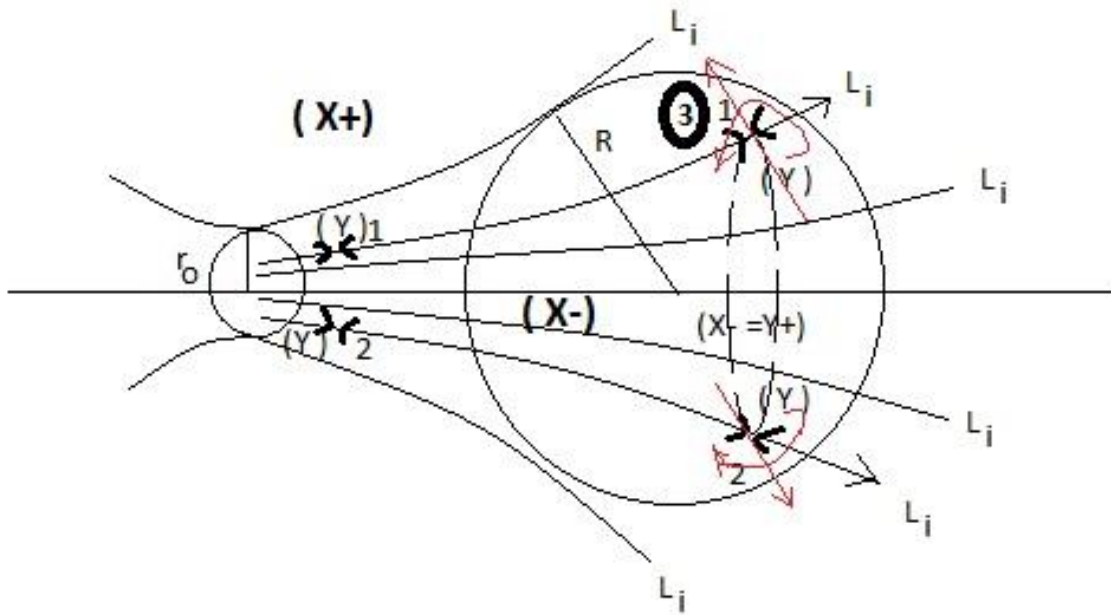
Fig. 3. Model of entangled particles.
