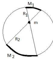
Fig.6. to the conditions of expansion of space-matter
