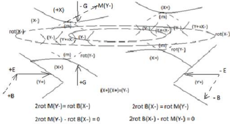
Fig. 9.2. Strong Interaction
