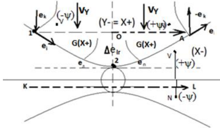
Fig. 7. Quantum gravitational ( X+ = Y- ) mass field.
