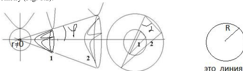
Fig. 1.2 Isotropic dynamics.
