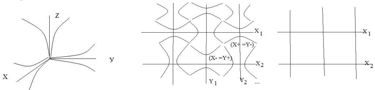
Fig.3 dynamic space-matter
