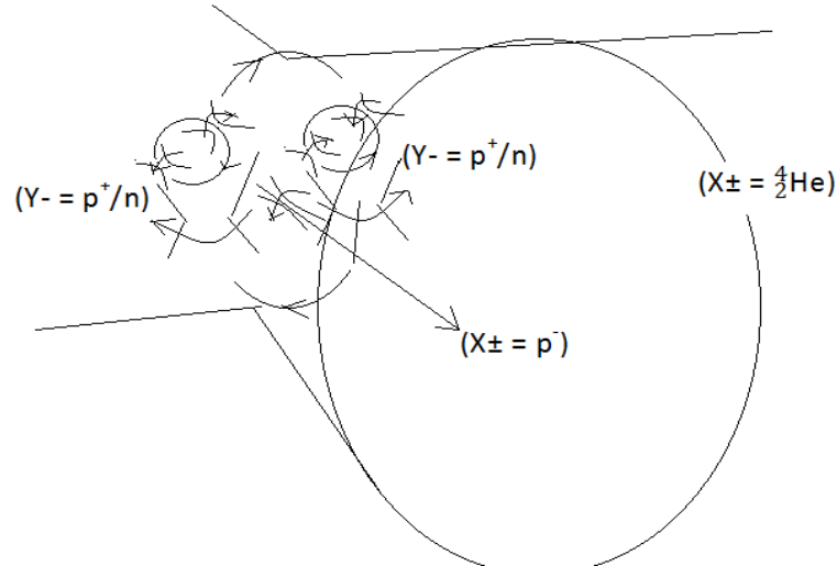
Figure1. Synthesis Model
