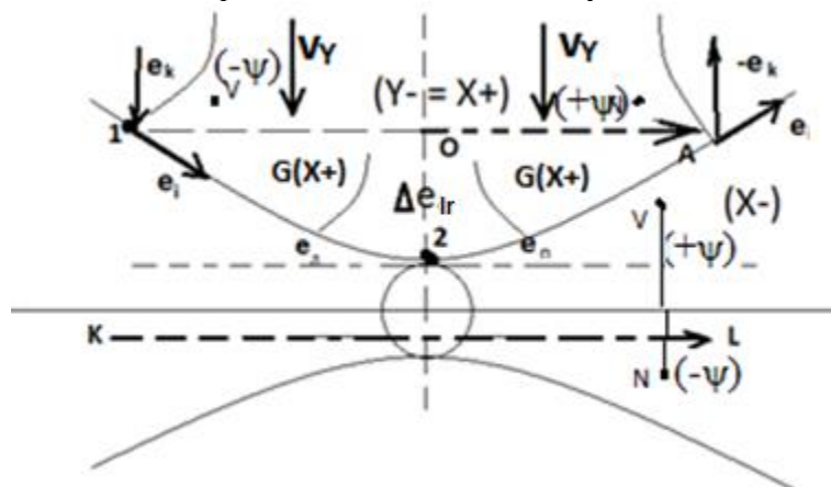
The physical property of the gravitational ( X+ = Y- ) mass field is the principle of equivalence of inertial and gravitational mass. This is the equality of acceleration a = v_Y * M(Y-) mass trajectories and acceleration g = G(X+) of the gravitational field, v_Y * M(Y-) = a = g = G(X+) , in velocity space
