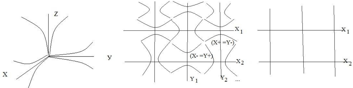
Fig.3 dynamic space-matter
