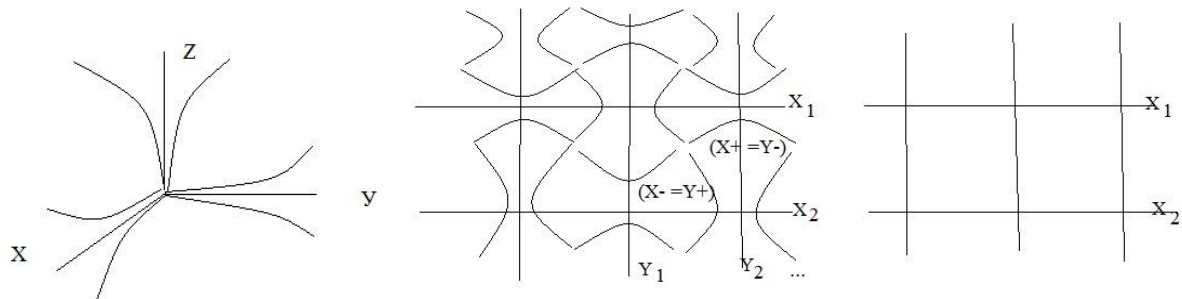
figure 3.3 dynamic space-matter
