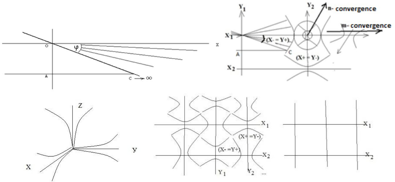
Fig. 1. Dynamic space-matter.
