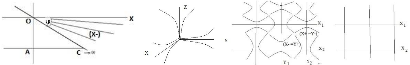
Figure 1. Dynamic space-matter.
