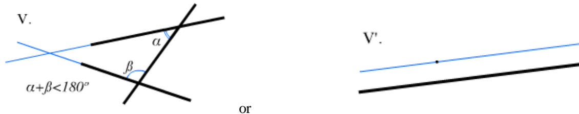
Figure 1 Euclidean axiomatic
