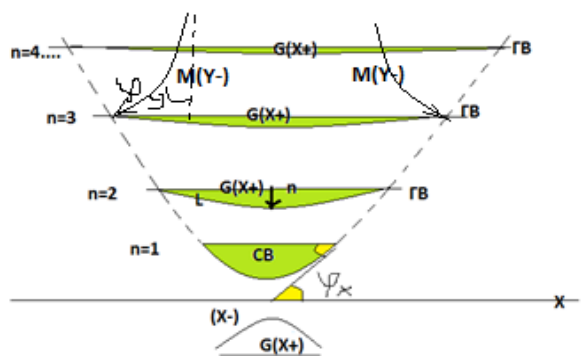
Fig. 4. Quantum gravitational fields.
