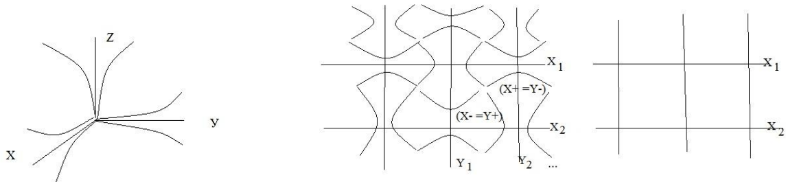
Fig.3 dynamic space-matter
