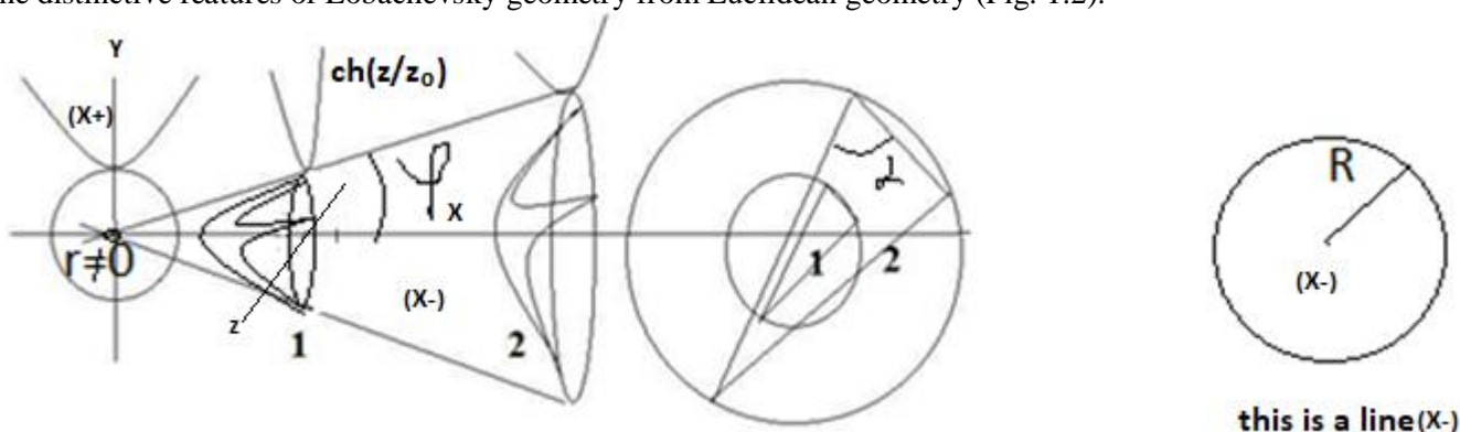
Fig. 1.2 Isotropic dynamics.
