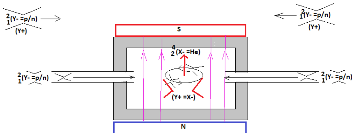
Fig.5.1 thermonuclear reactor.
