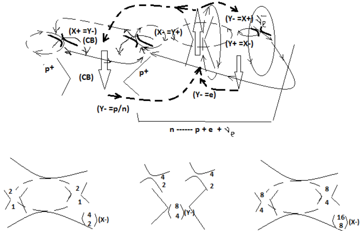
Based on these properties ( X = p^+ ) and ( X = \nu_e^- ), the decay time of a neutron in a strong ( X -)magnetic field should increase. This is verified in an experiment.
