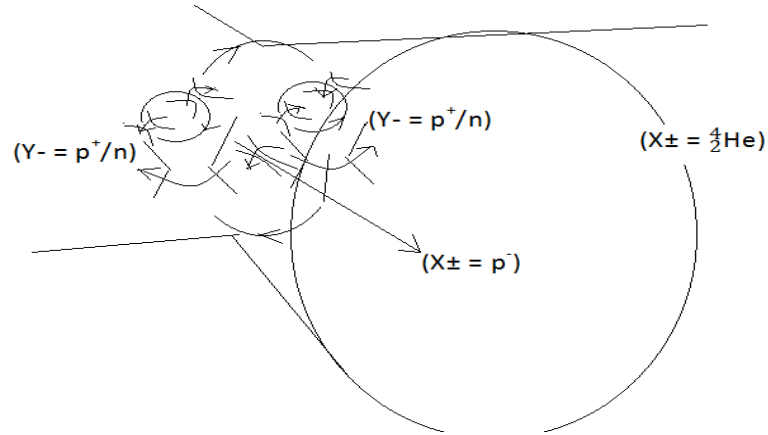
Fig.5.1 Synthesis model
