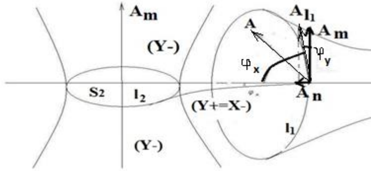
Fig. 2.2-1. Electromagnetic (Y+= X-)and gravitational (X+= Y-)fields.
