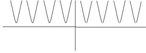
Fig.3.3. graph of the dynamics of quantum fields
