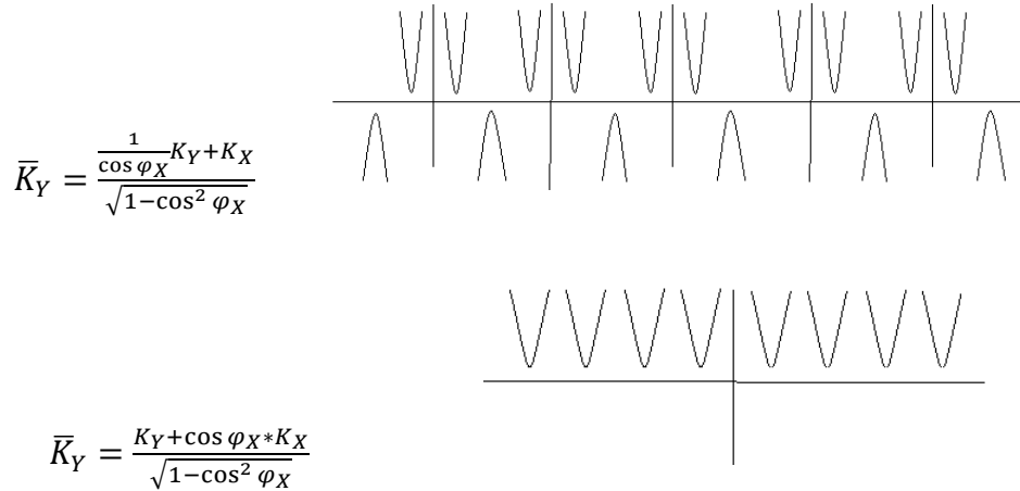
Fig.3.3. graph of the dynamics of quantum fields
