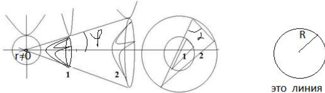
Fig. 1.2 Isotropic dynamics.
