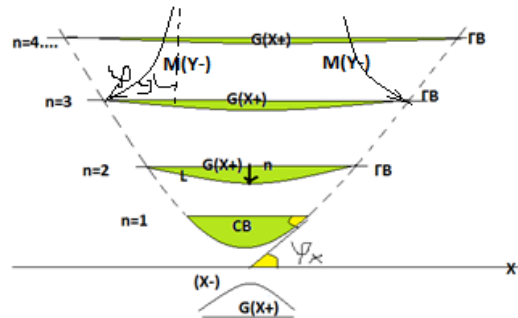
Fig. 4. Quantum gravitational fields.
