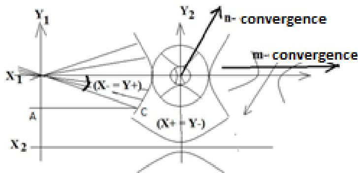
Fig. 3a. dynamic space-matter
