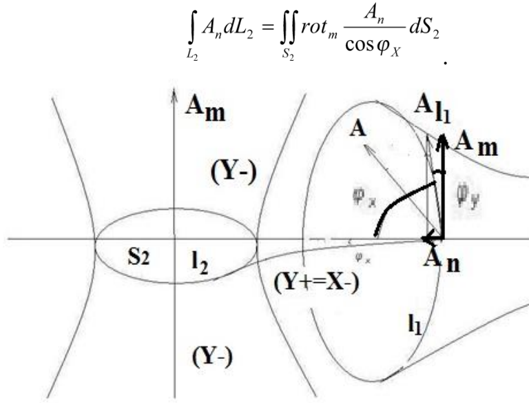
Fig. 2.2-1. Electromagnetic (Y+= X-) and gravitational (X+= Y-) fields.
