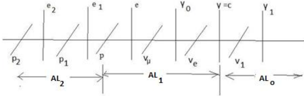
Figure 2. Indivisible quanta of space-matter.
