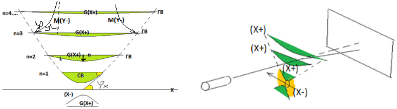
Fig. 5 Quantum gravitational fields
