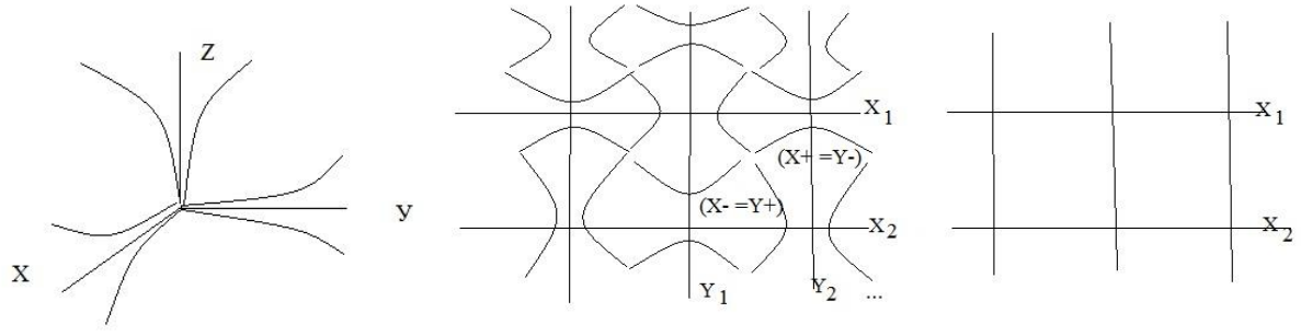
Fig.3 dynamic space-matter
