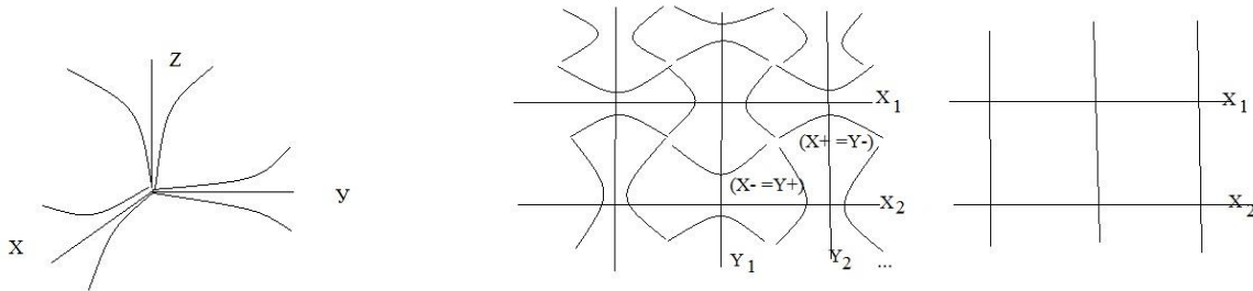
Fig.3 dynamic space-matter/
