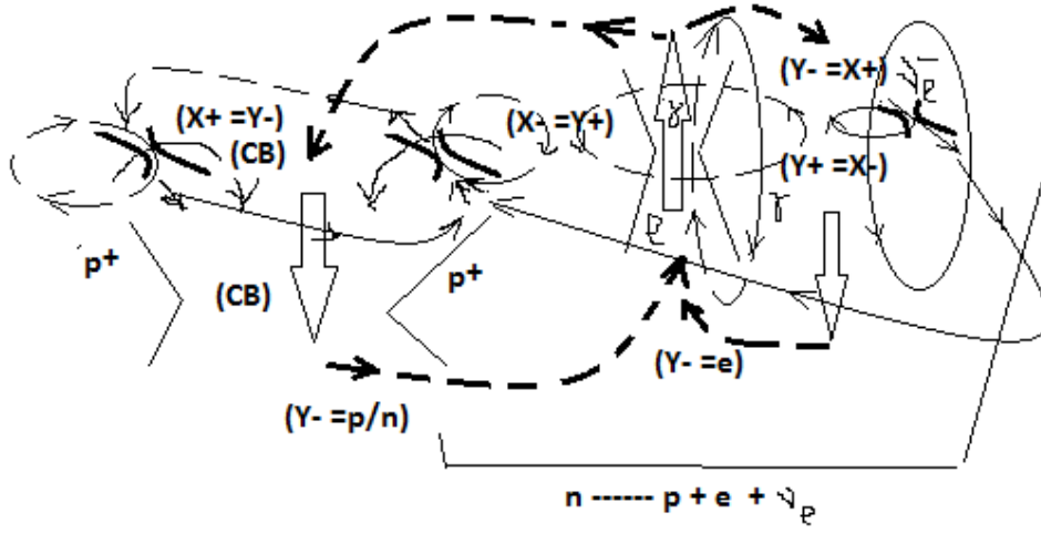
Figure 3.6. Quantum ( Y- = p/n ) and similar ( Y- = 2n ) Strong Interaction
