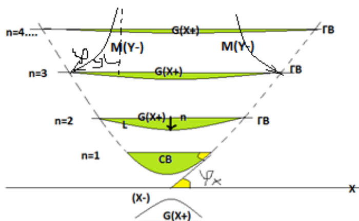
Fig . 4. Quantum gravity fields .
