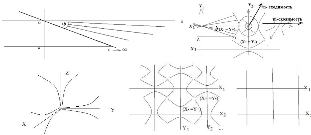
Fig. 1. Dynamic space-matter.
