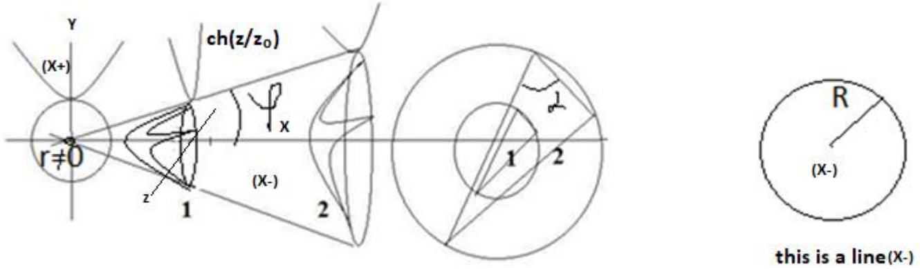
Fig. 1.2 Isotropic dynamics.
