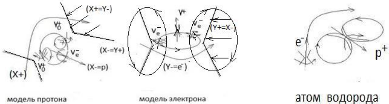
Fig. 3.3 Models of the products of proton-electron annihilation
