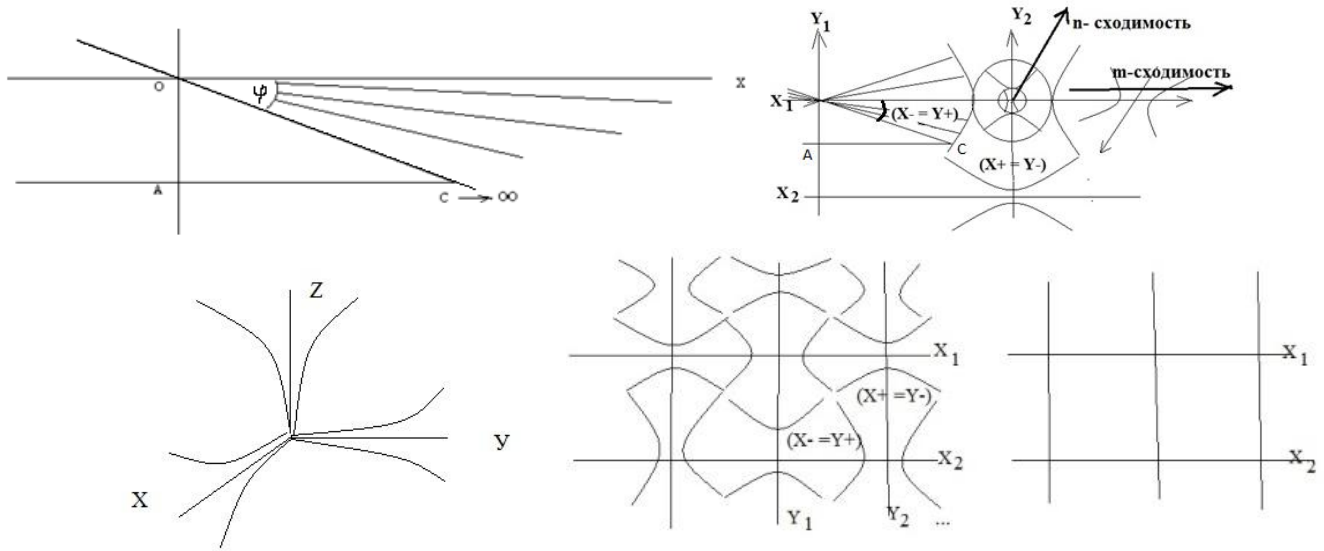
Figure 1. Dynamic space-matter.
