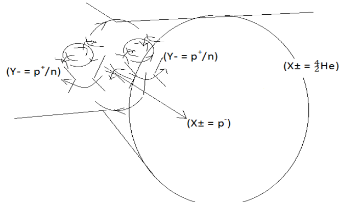
Fig.5.1 Synthesis model
