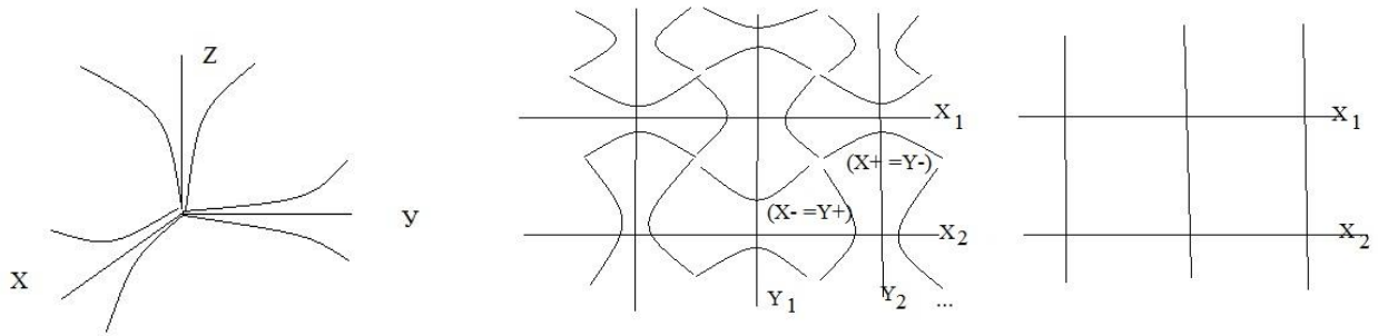
Fig.3 dynamic space-matter
