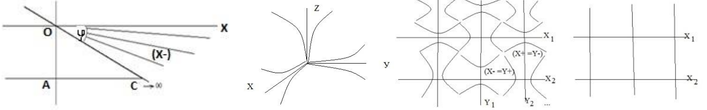
Figure 1. Dynamic space-matter.
