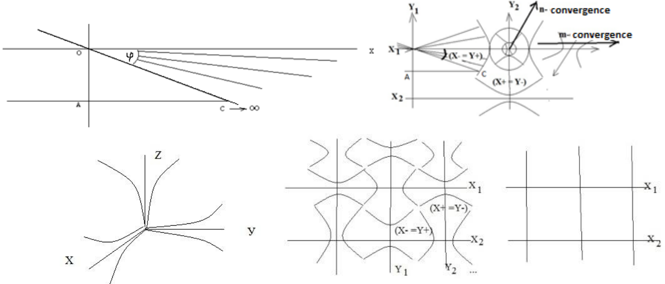
Fig. 1. Dynamic space-matter.
