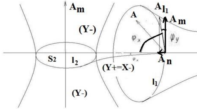
Figure 3. Electro (Y+=X-) magnetic and gravitational (X+=Y-) fields.
