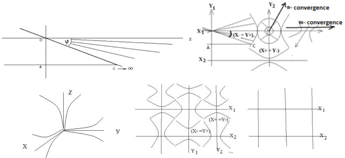
Fig. 1. Dynamic space-matter.
