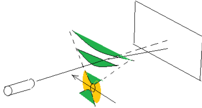
Fig. 4.1. Quantum gravity fields.
