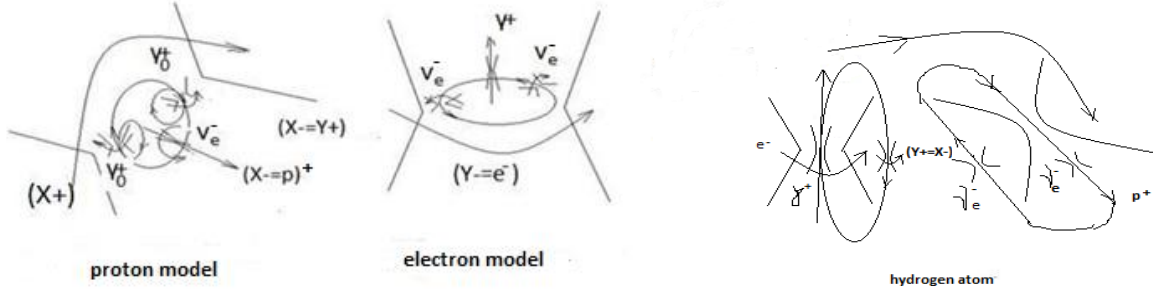
Fig. 5. Models of the products of proton and electron annihilation
