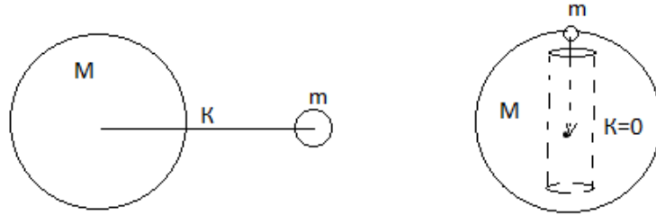
Fig.5. Newton's law
