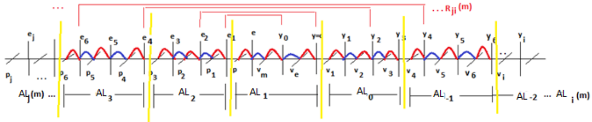
Fig.5. spectrum of indivisible quanta
