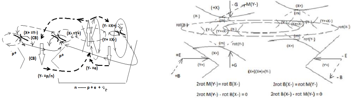
Fig.6.1. Quantum ( Y- = p/n ) and similar ( Y- = 2n ) Strong Interaction
