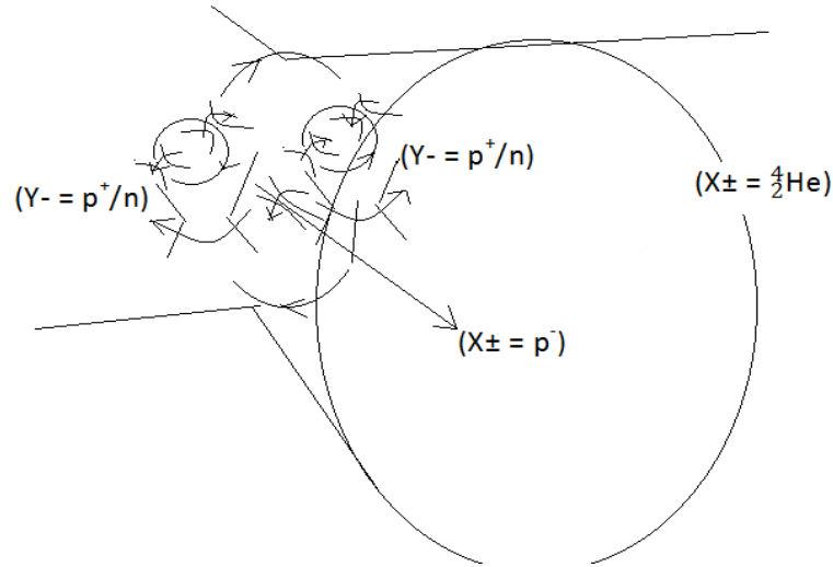
Figure1. Synthesis Model
