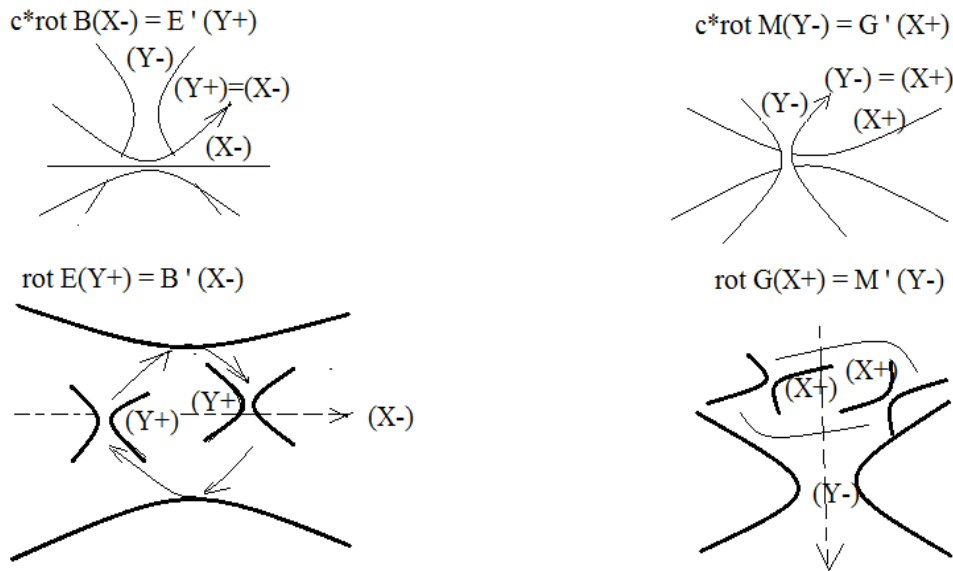
Figure 4. Unified fields of space-matter.
