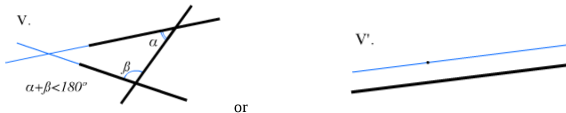
Figure 1 Euclidean axiomatic
