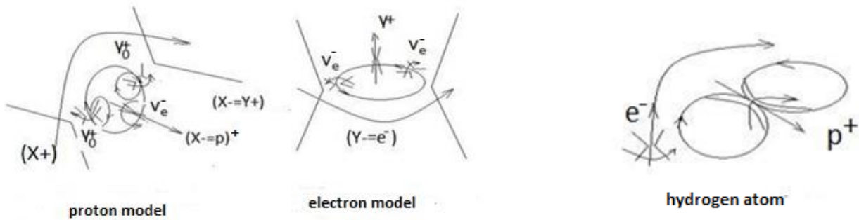
Figure 5. Models of the products of proton-electron annihilation
