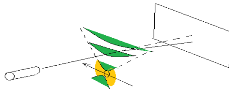
Fig. 4.1 Quantum gravitational fields.
