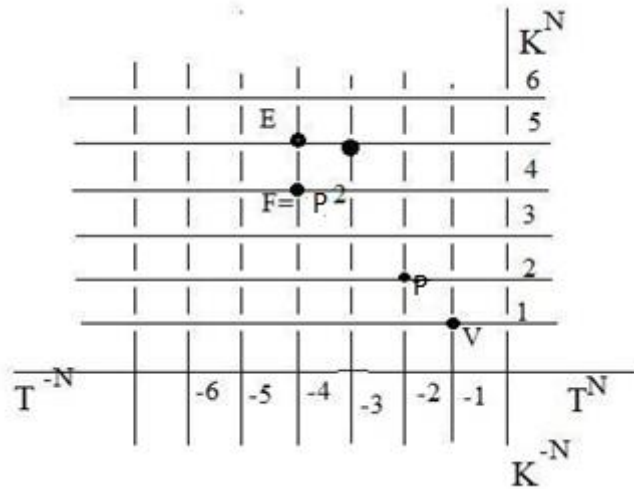
Fig.4 unified Criteria for the Evolution of space-matter.
