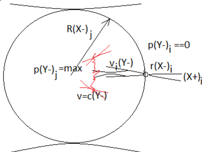
Fig.8b. to the dynamics of the space-matter of the Universe In quantum gravity, the acceleration of mass trajectories (Y- = X+) in a gravitational field
