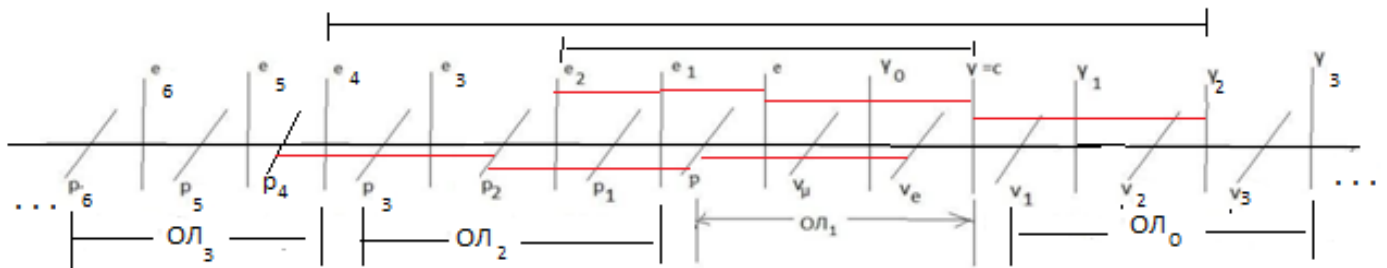
Fig.4 quantum coordinate system
