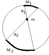
Fig.6. to the conditions of expansion of space-matter velocity of the masses ( M_1 ) and ( M_2 ), relative to the mass of the observer ( m ):
