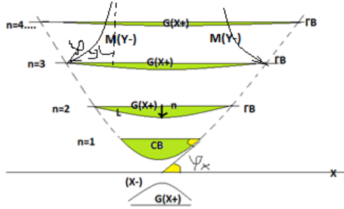
Fig. 5.3. Quantum gravity fields.
