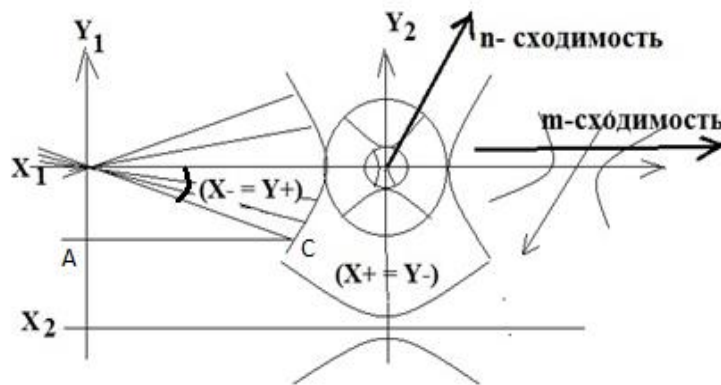
Fig. 3a. dynamic space-matter
