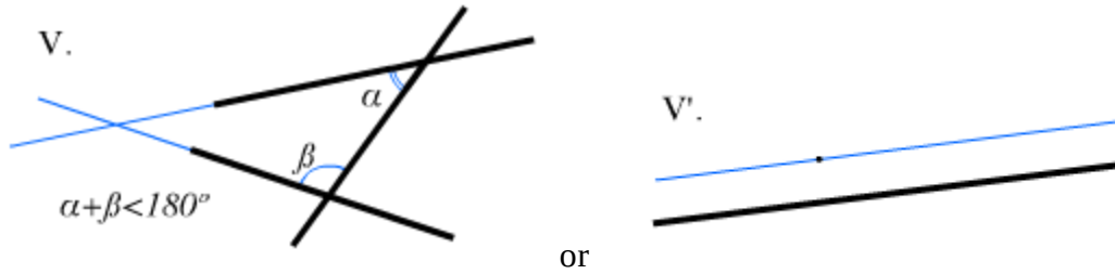
or drawing. 3.1 Euclidean axiomatics
