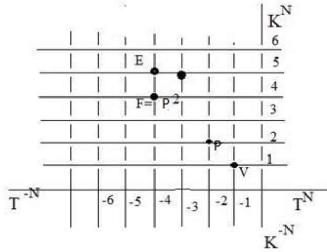
Fig.4 unified Criteria for the Evolution of space-matter.
