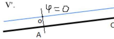
rice. 1 Euclidean axiomatics .
