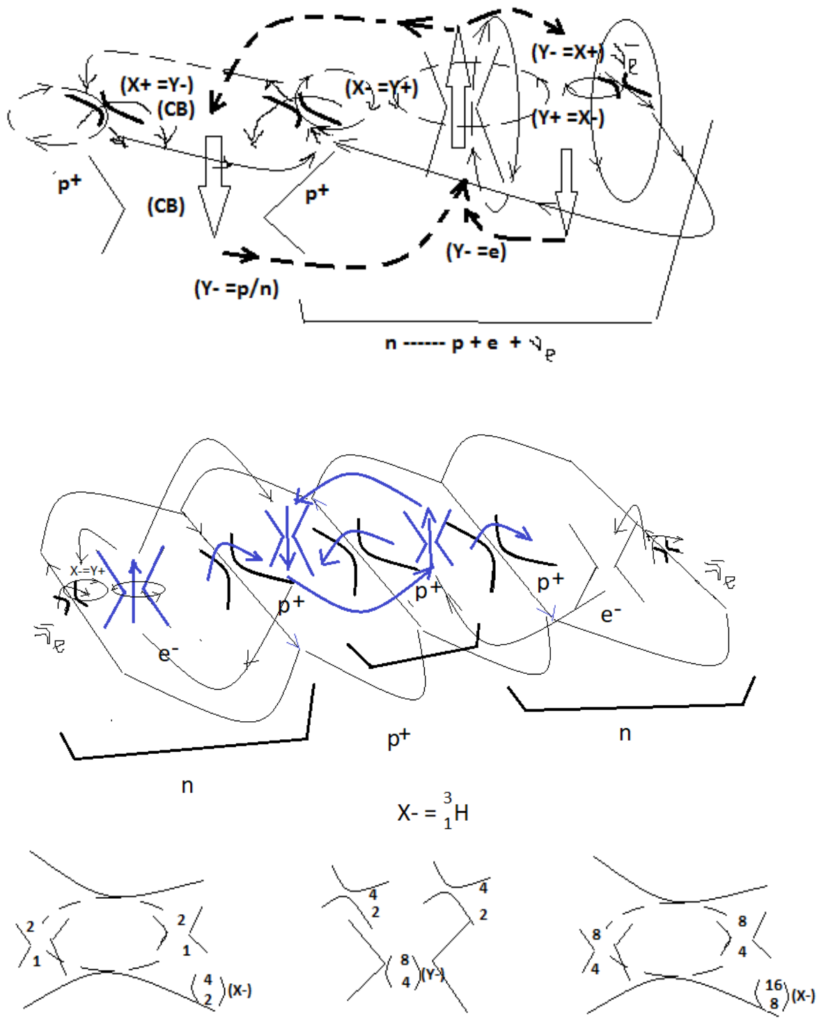
Fig. 9.1. Quantum ( Y^- = p/n ) and similar ( Y^- = 2n ) Strong Interaction Based on these properties ( X^- = p^+ ) and ( X^- = \bar{\nu}_e ), the decay time of a neutron in a strong ( X^- ) magnetic field should increase. This is verified in an experiment.
