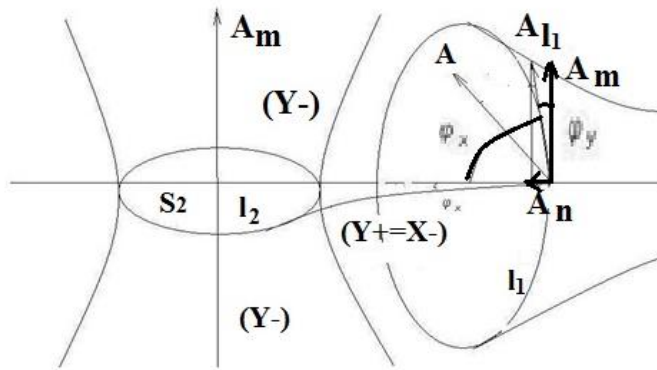
Figure 3. Electro ( Y+ = X- )magnetic and gravitational ( X+ = Y- )fields.
