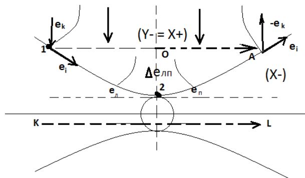
Figure 6a. Quantum of space-matter
