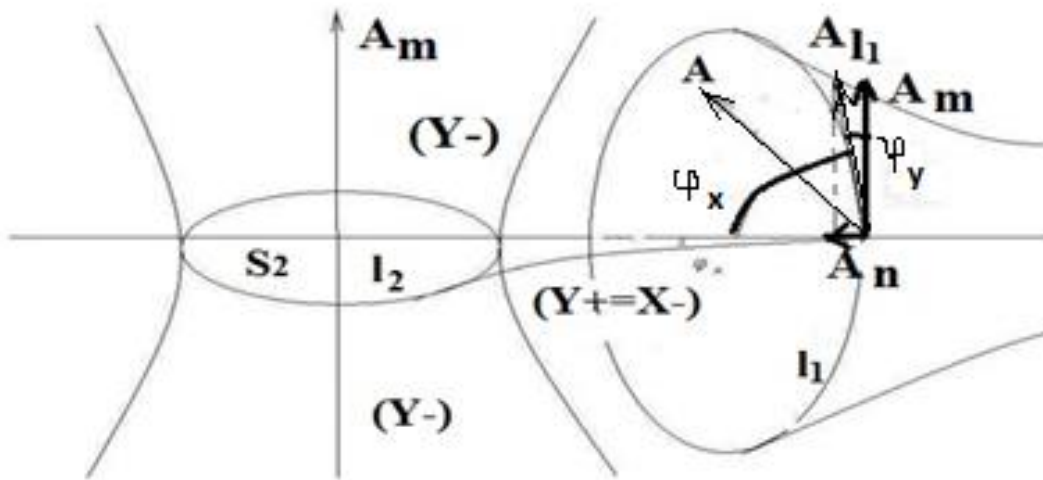
Fig. 2.2-1. Electromagnetic ( Y+=X- ) and gravitational ( X+=Y- ) fields.
