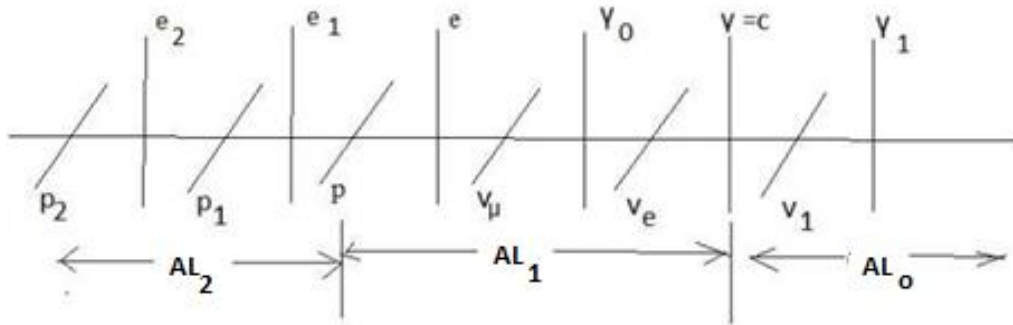
Figure 2. Indivisible quanta of space-matter.
