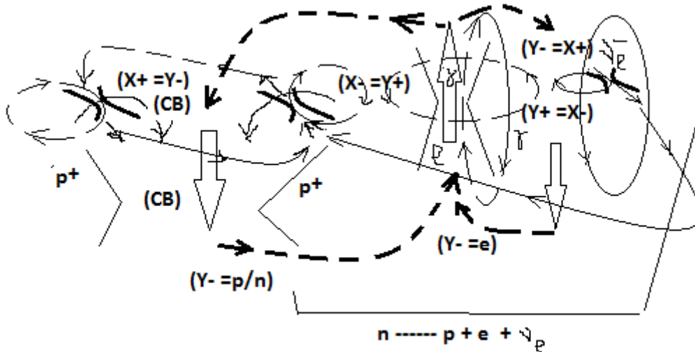
Figure 3.6. Quantum (Y- = p/n) and similar (Y- = 2n) Strong Interaction
