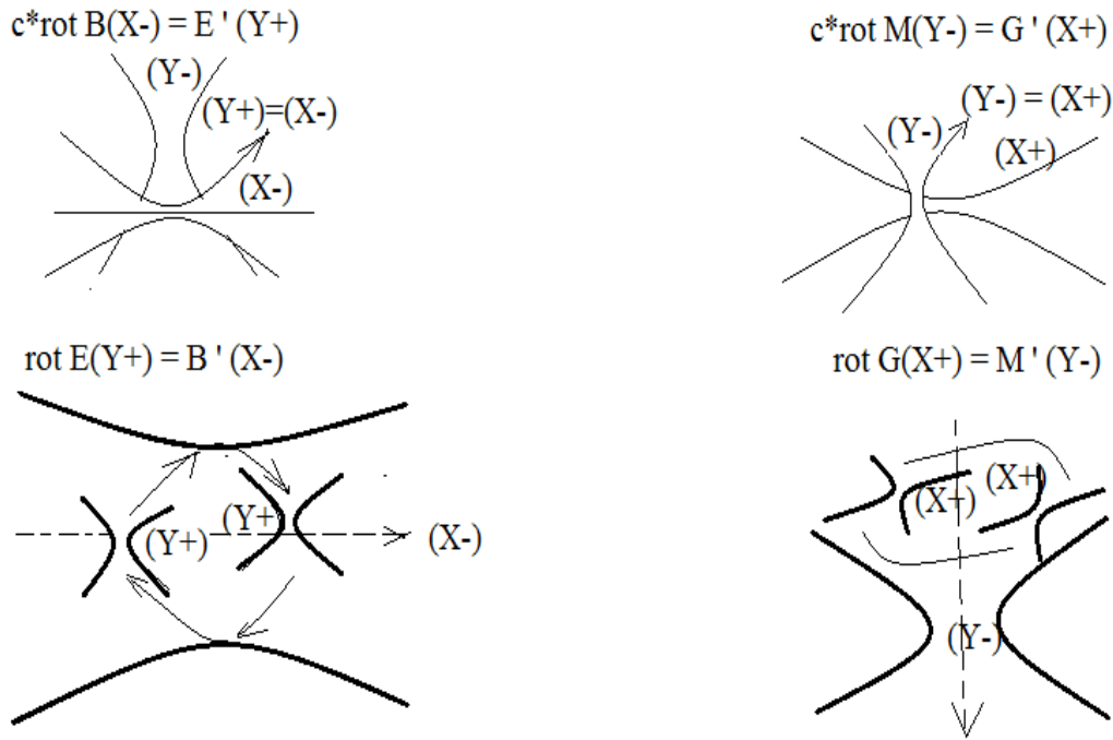
Fig.2.2-2. Unified fields of space-matter
