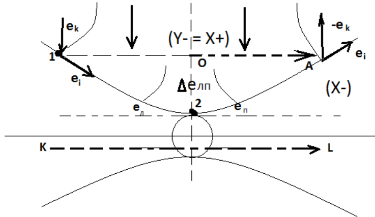
Figure 6. Quantum of space-matter
