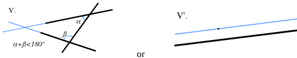
rice. 2 Euclidean axiomatics
