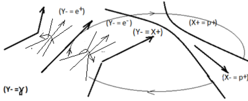
Fig. 7 birth of an electron-positron pair
