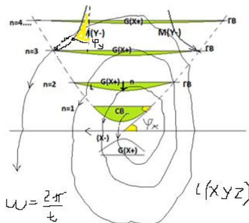
Figure 8. Quantum gravitational fields.
