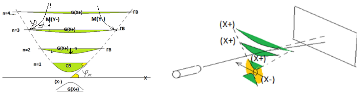
Fig. 5 Quantum gravitational fields
