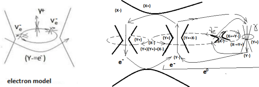
Figure 9. Allowable structures of leptons.
