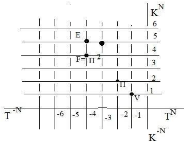
Figure 7. Criteria of Evolution in space-time.
