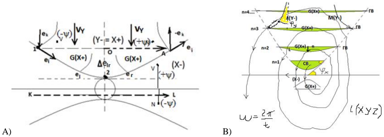
Figure 6. Strong and Gravitational Interaction
