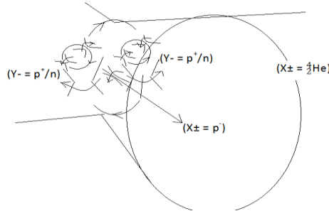
Figure1. Synthesis Model
